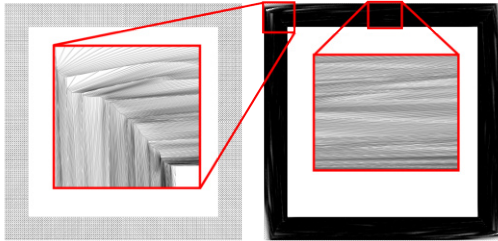
Fig. 4. A stress test that our method passes. We rotate the inner rectangle by \pi , setting the inner and outer rectangles as positional constraints. A bijective mapping will inevitably undergo an extreme amount of distortion. The zoom-in views show that the triangles become very thin: Successful maps must avoid “geometric locking” that possibly prevent any solution, which is not a concern in the smooth setting. This example suggests that the injective mapping problem can have more of a combinatoric nature rather than mimicking behaviors of smooth PDEs.
